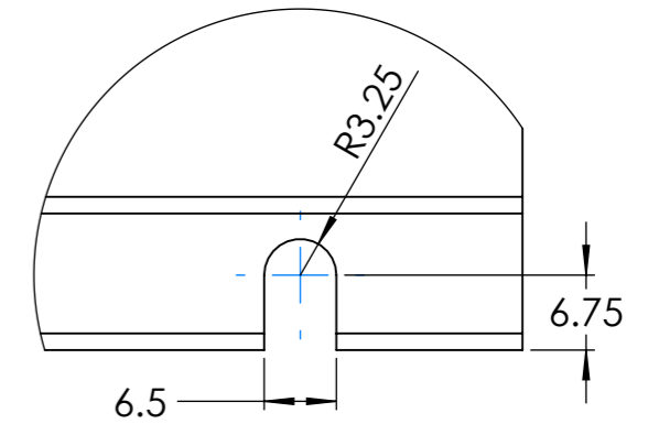
DETAIL A SCALE 2 : 1.5
